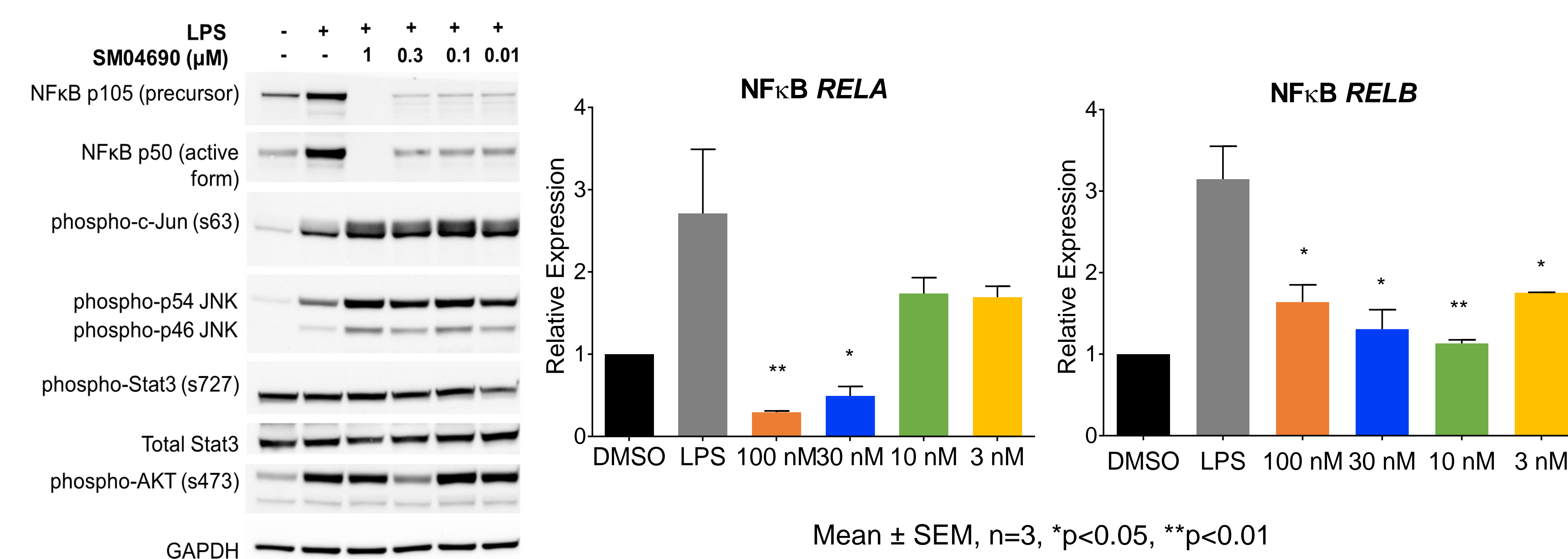
Figure 2. SM04690 specifically inhibited NF \kappa B phosphorylation and expression in vitro .
