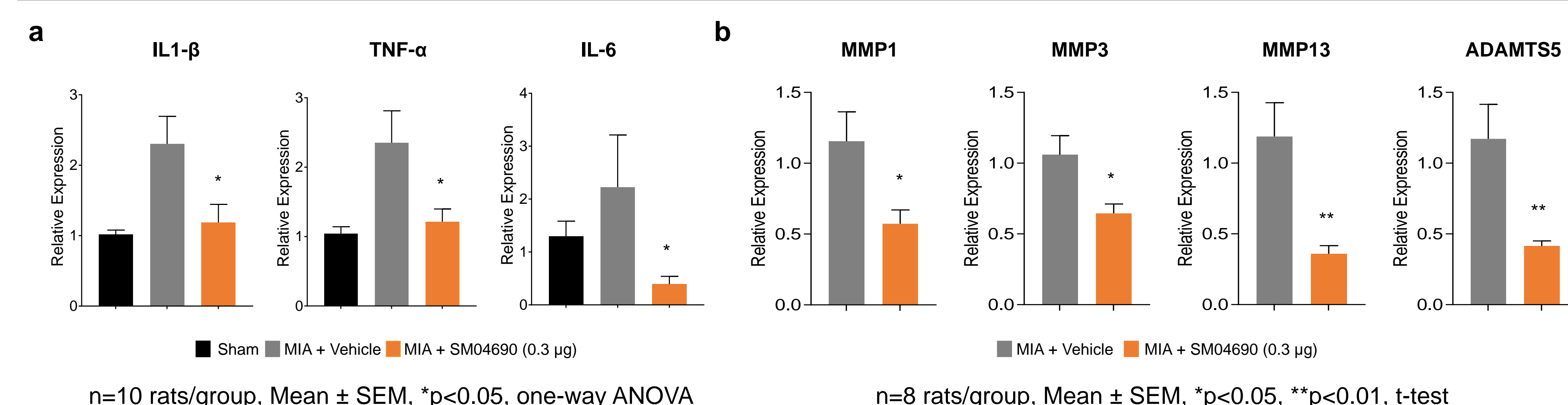
Figure 3. Single IA injection of SM04690 decreased inflammatory cytokines (a) and matrix metalloproteinases (MMPs) (b) compared with vehicle at Day 11.
