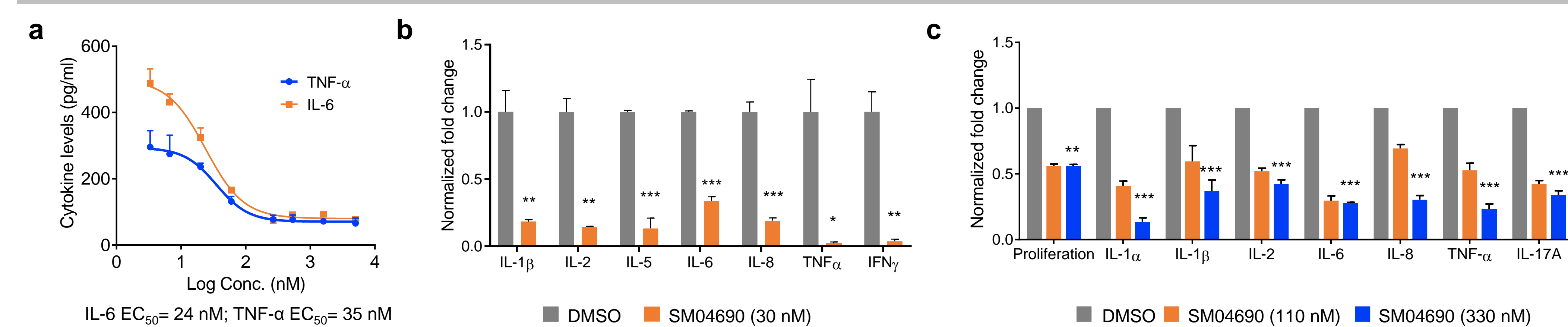
Figure 1. Synovial fibroblasts: dose-dependent inhibition of IL-6 (a) and TNF- \alpha (a) production demonstrated in both cell types. SM04690 inhibited pro-inflammatory cytokine secretion compared with vehicle as shown in (b) and (c) (n=3 replicates, mean \pm SEM, *p<0.05, **p<0.01, ***p<0.001).
