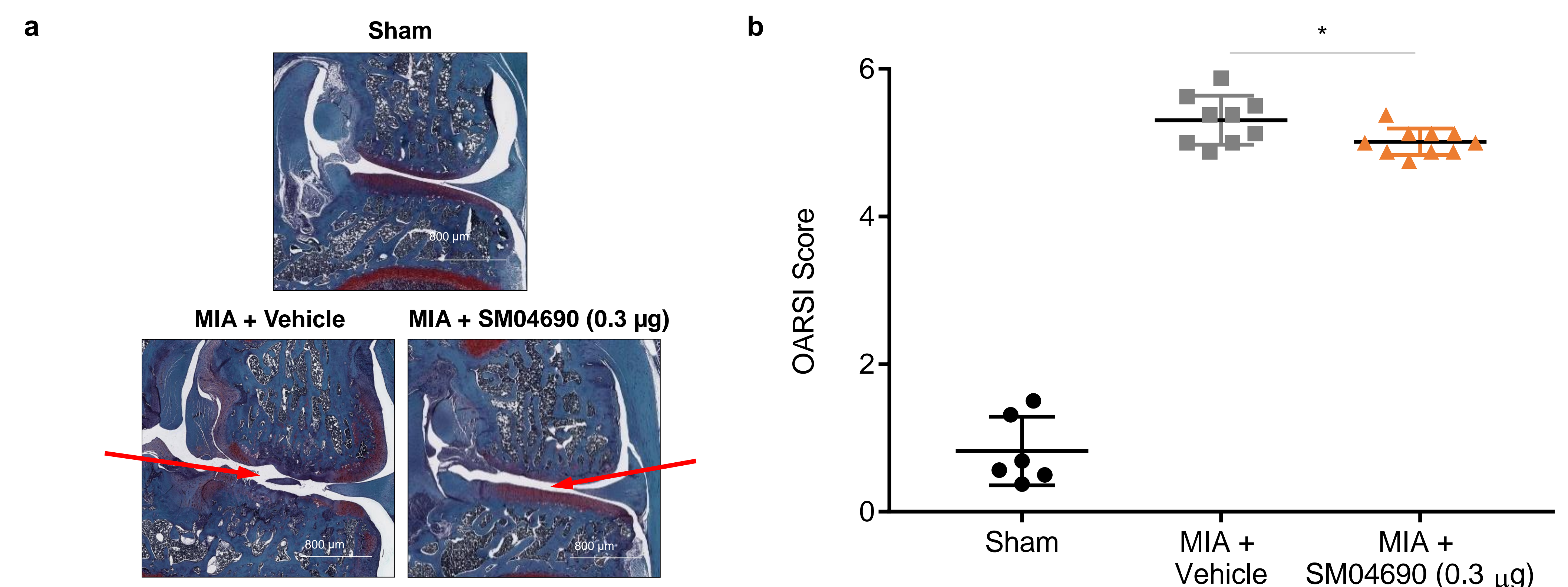
Figure 5. Single IA injection of SM04690 improved Safranin-O staining (a) and OARSI scores (b) at Day 28 comparing treatment with vehicle (n= 10, Mean \pm SD, *p<0.05, Mann-Whitney U test).
